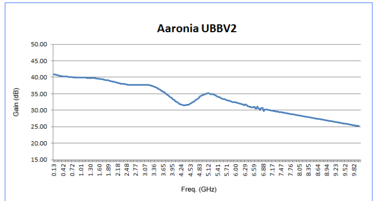
Gain UBBV2
